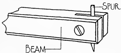
FIG. 338. GAGE FOR INLAY WORK.
